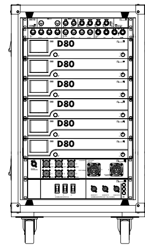
Z5576.xxx 6 x D80 Touring rack assembly OUT: 2 x LKA25F / 6 x NL8
