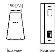
Vi10P cabinet dimensions in mm [inch]
