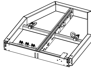
Z5380 V Flying frame For a maximum of twenty four V8/V12/Vi8/Vi12 loudspeakers or fourteen V/Vi subwoofers
