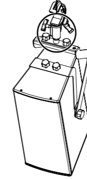
Yi7P/Yi10P with Z5399 YP Mounting bracket Z5010 TV Spigot with fixing plate Z5012 Pipe clamp
