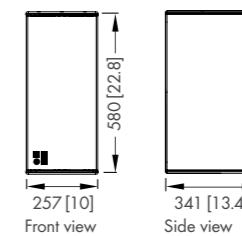
Front view Side view
